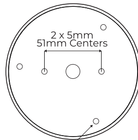
3 holes x 96 PCD to accept No 6 self tap screw (external fitting)
